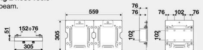
P/N 843013 Bracket for installing 3 hose reels 430 Series on HEA beam.
